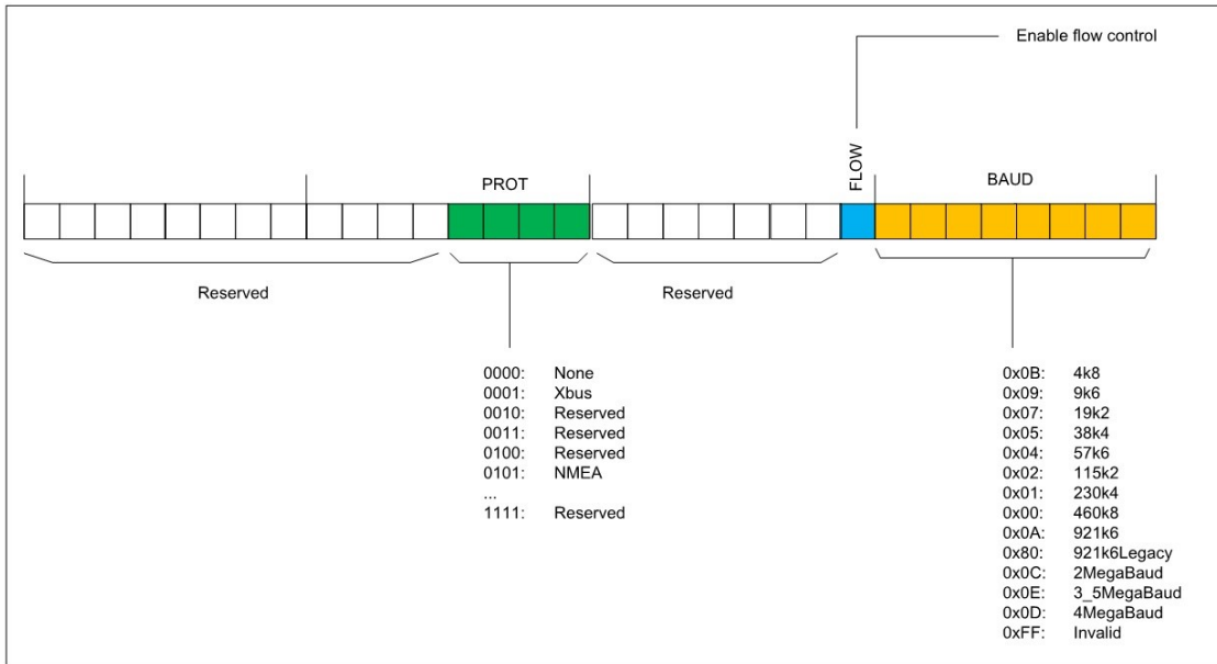
Figure 2: Port Configuration
